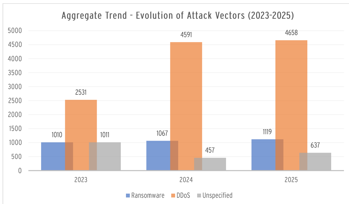
Figure 2: Illustrates the aggregate volume of recorded incidents for Ransomware and DDoS attacks from 2023 to 2025. The chart highlights a distinct divergence in growth patterns, comparing the volatility of disruptive attacks (DDoS) against the linear progression of extortion attempts (Ransomware).
