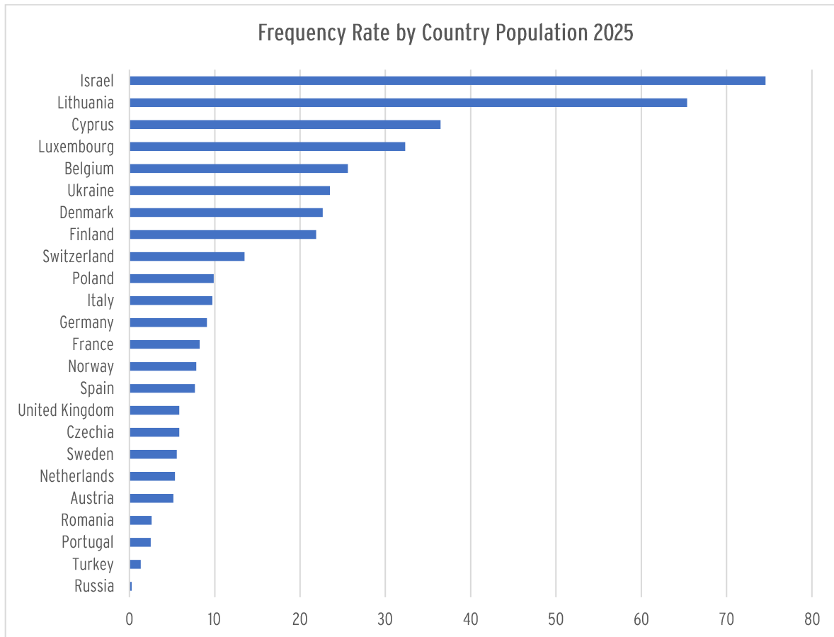
Figure 1: Displays the distribution of cyberattacks across the top 24 attacked European and strategically relevant neighbouring countries in 2025, measured per million inhabitants. This metric normalises the incident volume against population size to identify regions with the highest relative threat intensity.
